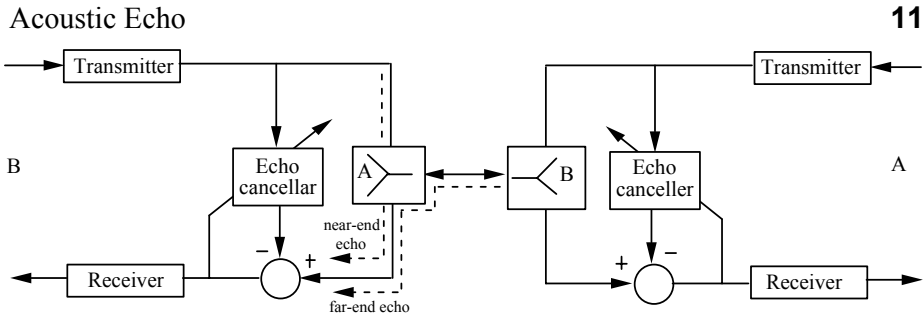
Figure 14.7 Echo cancellation in digital modems using 2-wire subscriber's loop.
