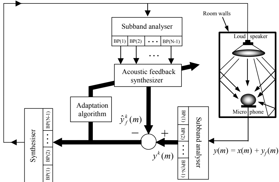
Figure 14.11 Configuration of a subband acoustic echo cancellation system.
