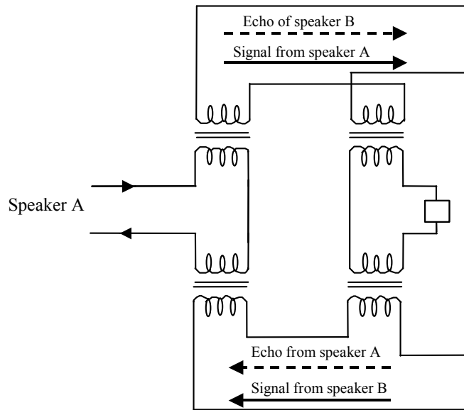
Figure 14.3 A 2-wire to 4-wire hybrid circuit.
