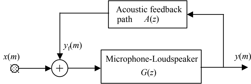
Figure 14.8 Configuration of a feedback model for a microphone–loudspeaker–room system.
